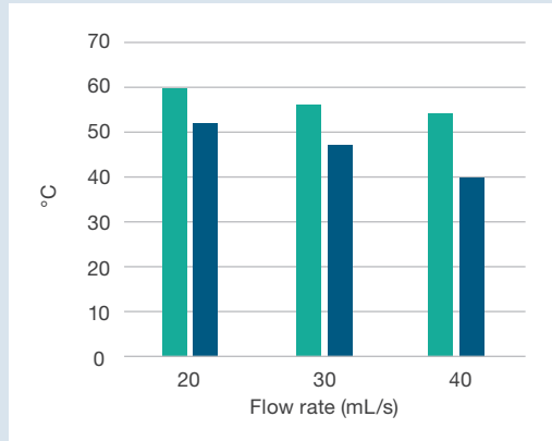
Figure 3 Comparing thermal properties of a cold-plate cooled system versus an immersion cooled system. Data generated from the physical rig set up.
