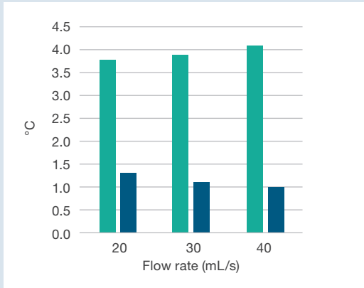
Figure 3 Comparing thermal properties of a cold-plate cooled system versus an immersion cooled system. Data generated from the physical rig set up.
